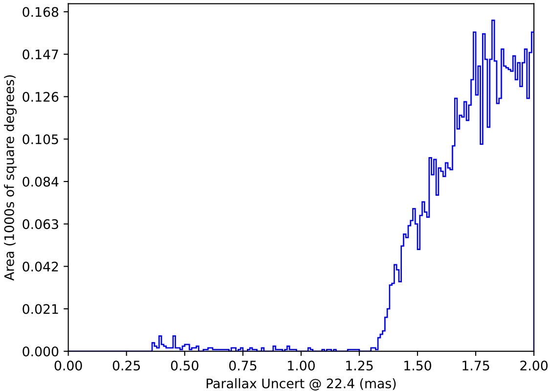
ddf_loaded_half_fl15_v3.4_10yrs : Parallax Uncert @ 22.4
