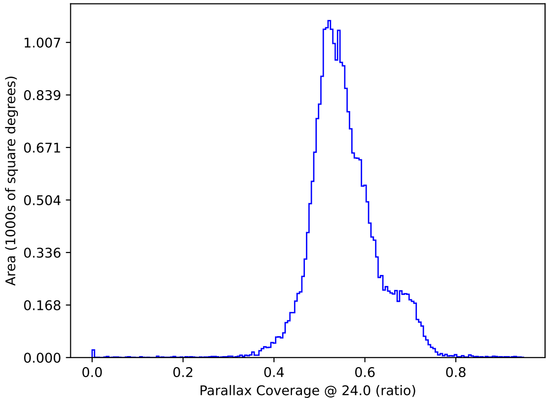
ddf_loaded_half_fl15_v3.4_10yrs : Parallax Coverage @ 24.0
