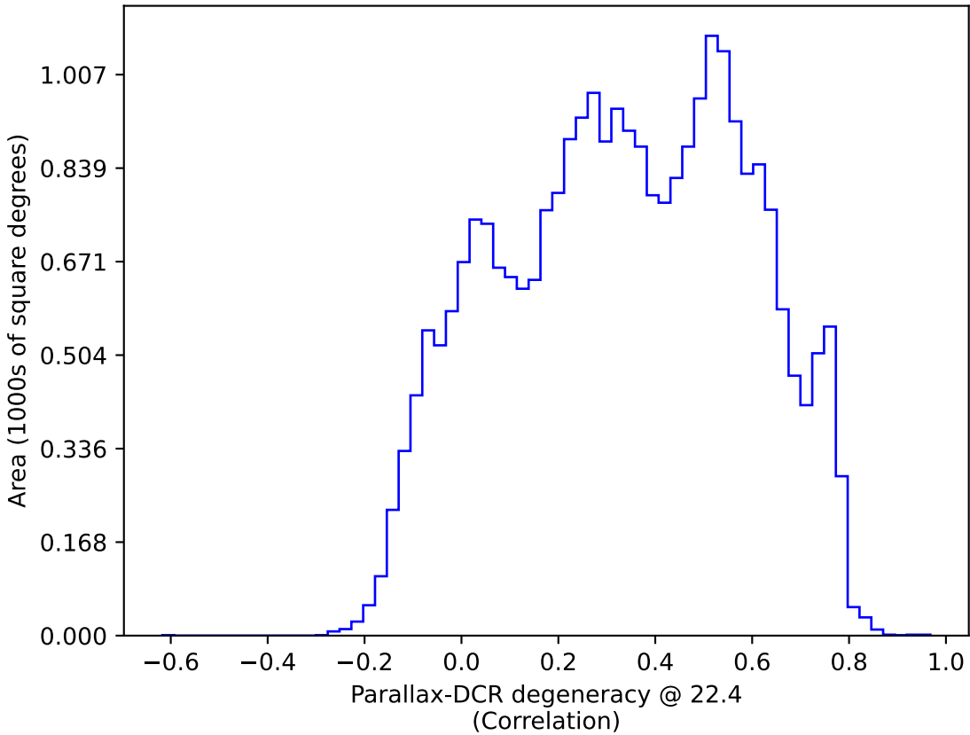
ddf_loaded_half_fl15_v3.4_10yrs : Parallax-DCR degeneracy @ 22.4
