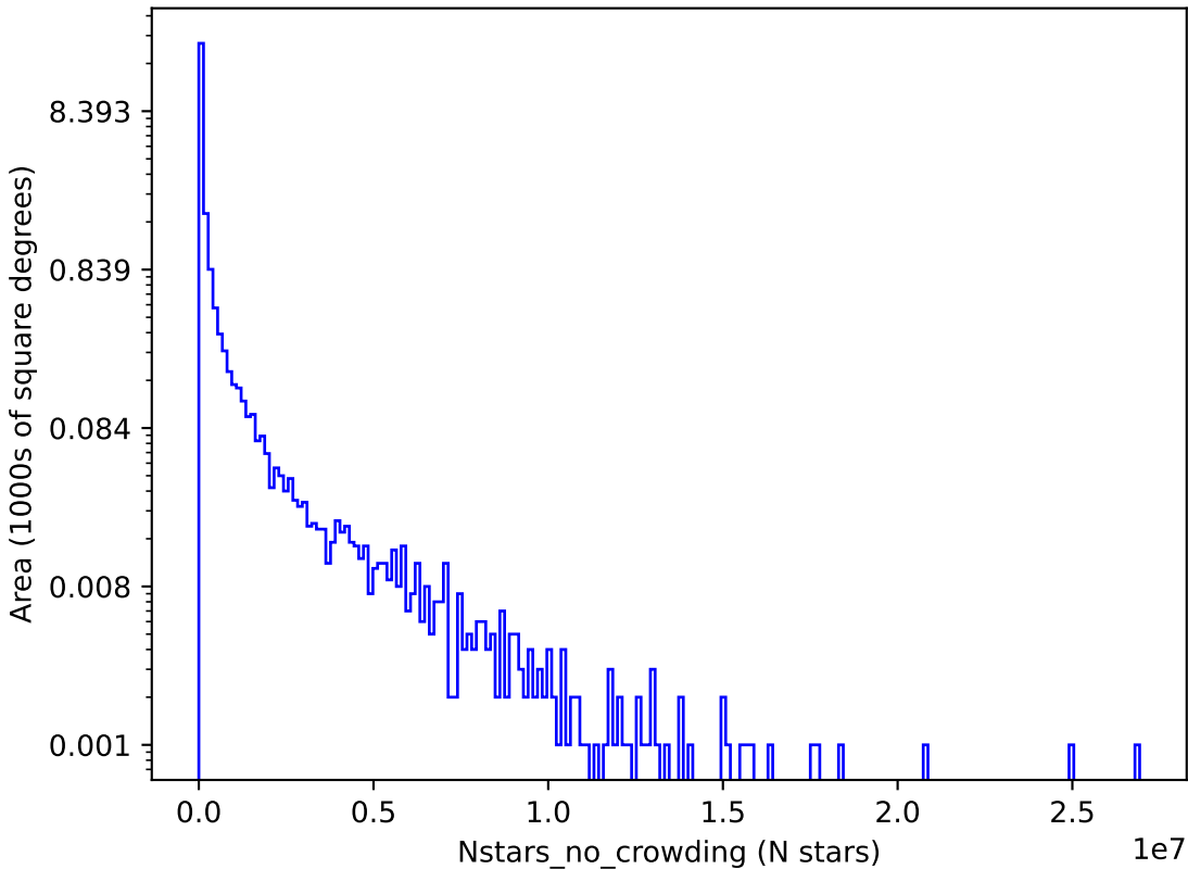
ddf_loaded_half_fl15_v3.4_10yrs z: Nstars_no_crowding
