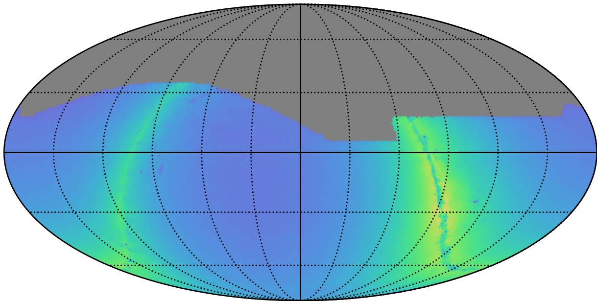
ddf_loaded_half_fl15_v3.4_10yrs r: Nstars_no_crowding
