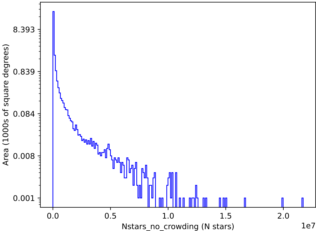
ddf_loaded_half_fl15_v3.4_10yrs r: Nstars_no_crowding
