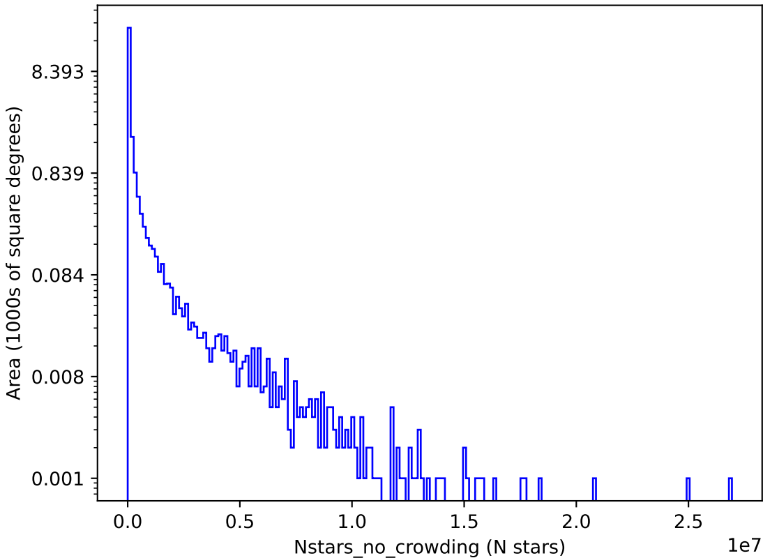
ddf_loaded_half_fl15_v3.4_10yrs i: Nstars_no_crowding
