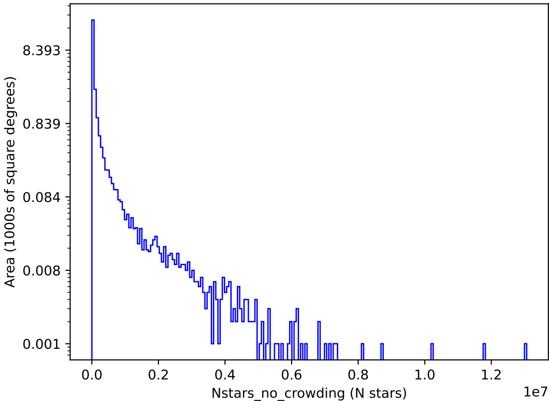
ddf_loaded_half_fl15_v3.4_10yrs g: Nstars_no_crowding
