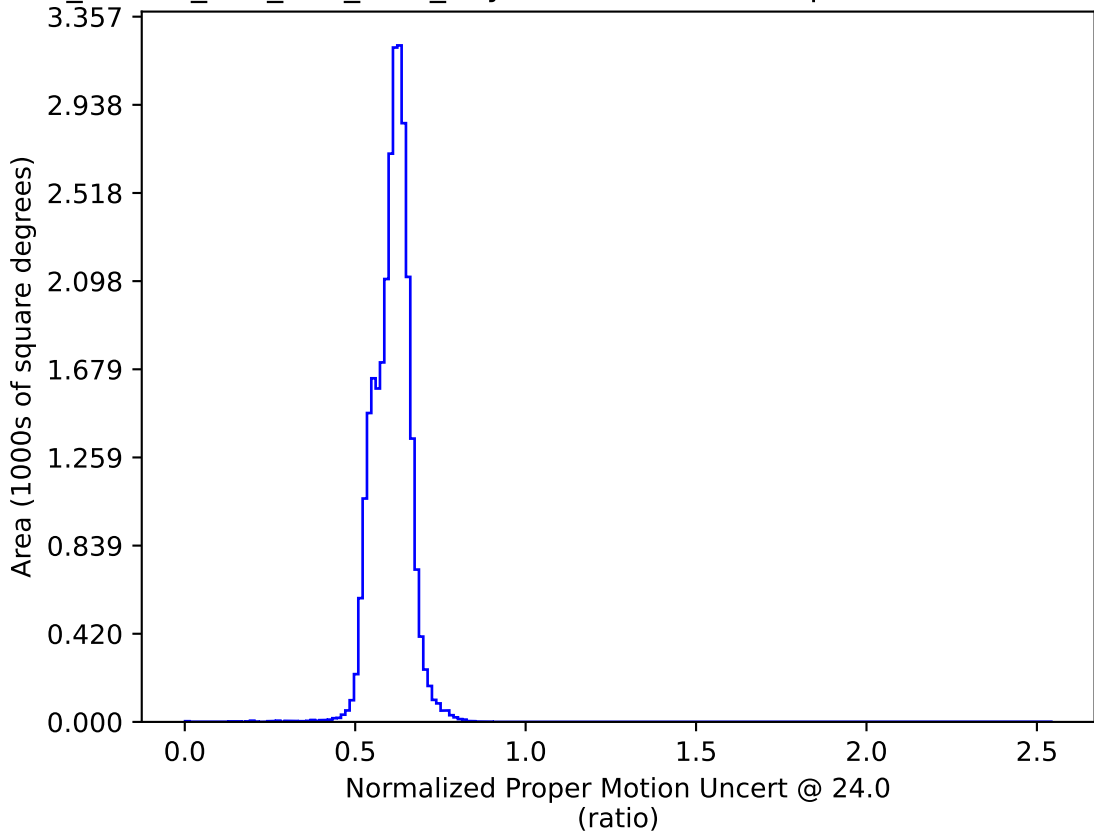
ddf_loaded_half_fl15_v3.4_10yrs : Normalized Proper Motion Uncert @ 24.0
