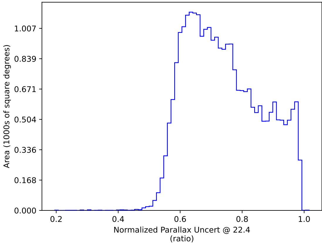
ddf_loaded_half_fl15_v3.4_10yrs : Normalized Parallax Uncert @ 22.4
