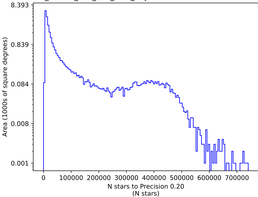
ddf_loaded_half_fl15_v3.4_10yrs z: N stars to Precision 0.20
