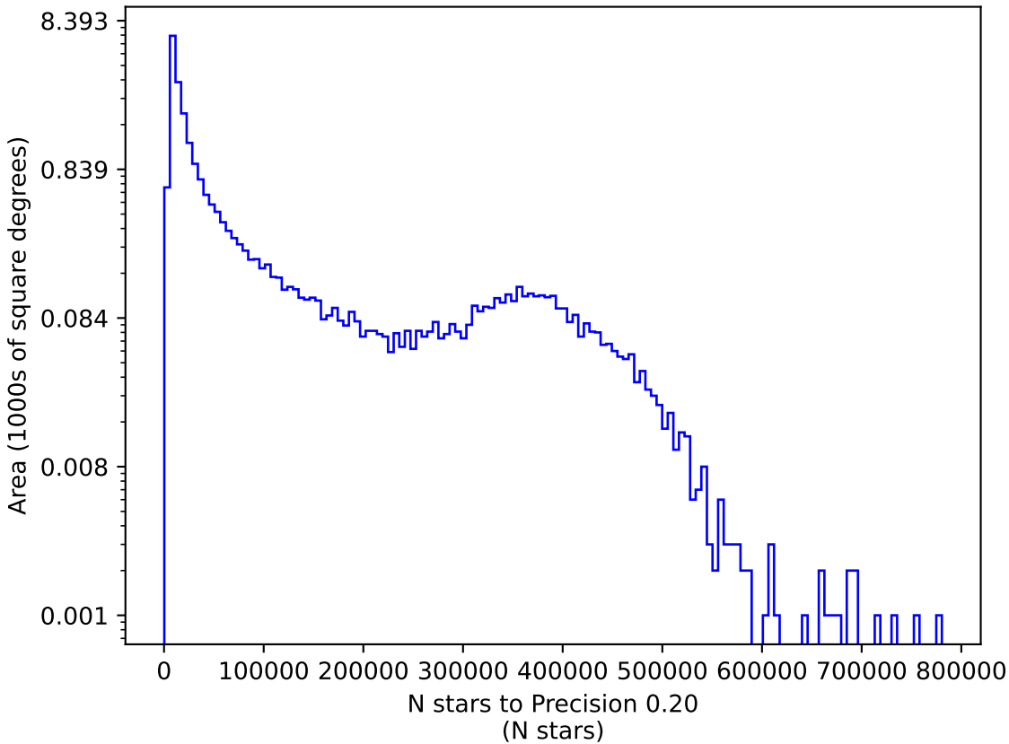
ddf_loaded_half_fl15_v3.4_10yrs y: N stars to Precision 0.20
