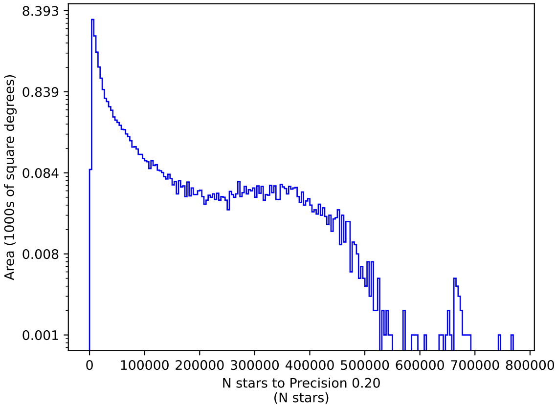
ddf_loaded_half_fl15_v3.4_10yrs g: N stars to Precision 0.20
