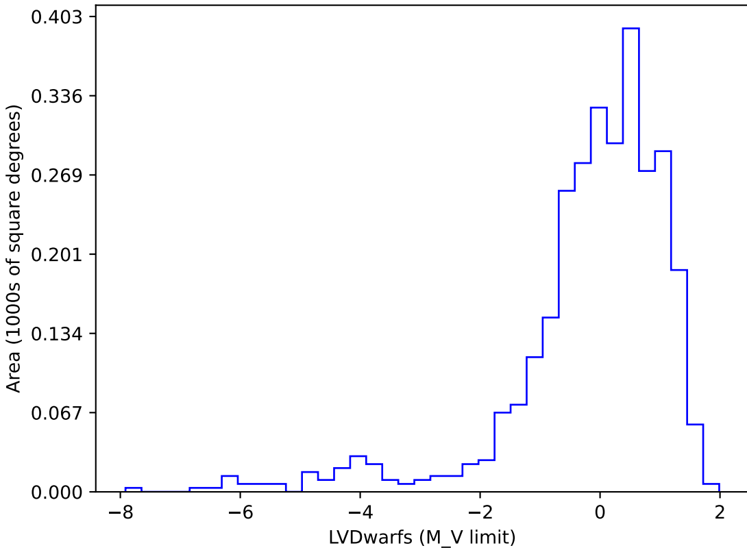
ddf_loaded_half_fl15_v3.4_10yrs gi SCP: LVDwarfs
