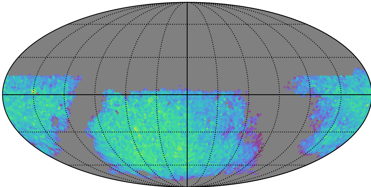
ddf_loaded_half_fl15_v3.4_10yrs gi: LVDwarfs
