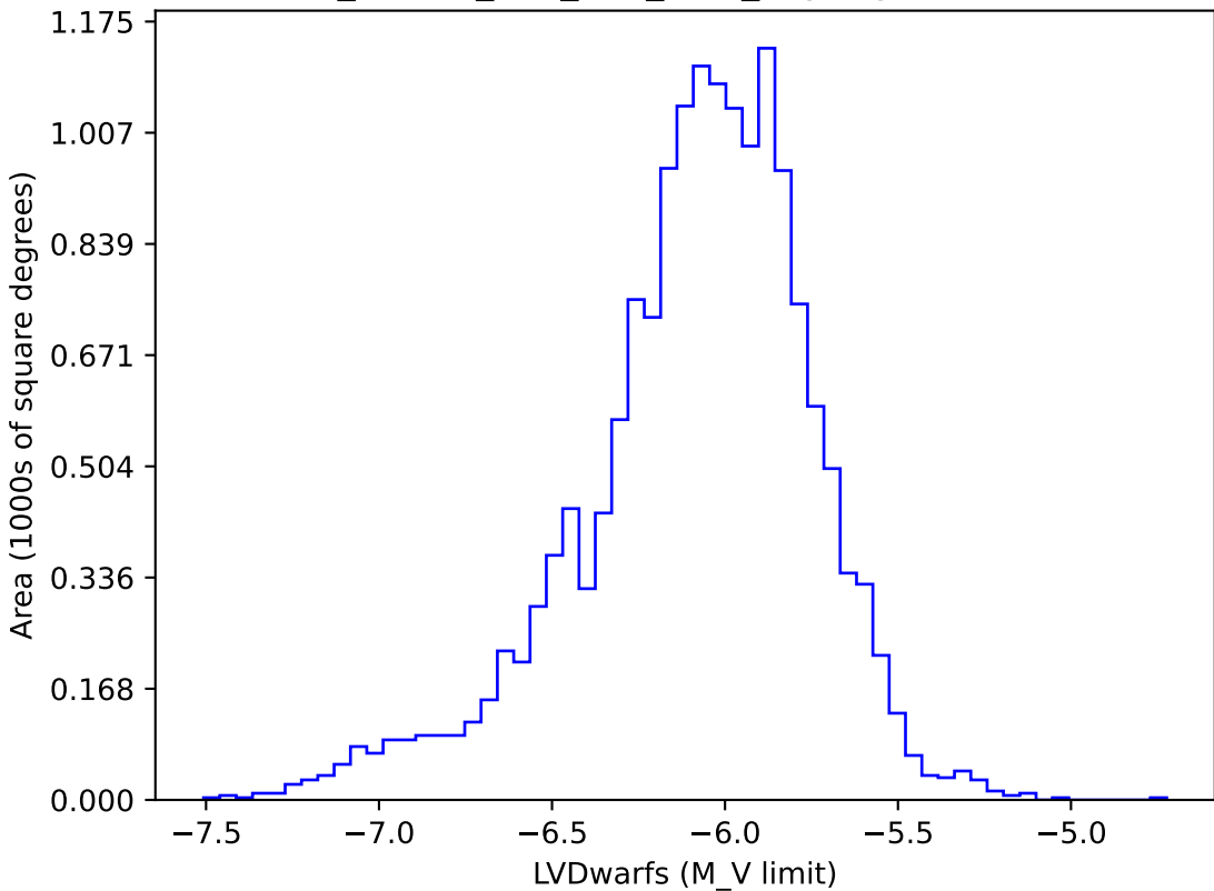
ddf_loaded_half_fl15_v3.4_10yrs gi: LVDwarfs
