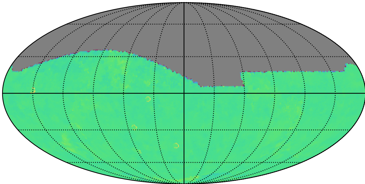
ddf_loaded_half_fl15_v3.4_10yrs z: Kuiper rotTelPos
