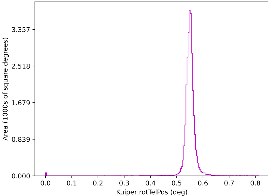
ddf_loaded_half_fl15_v3.4_10yrs z: Kuiper rotTelPos
