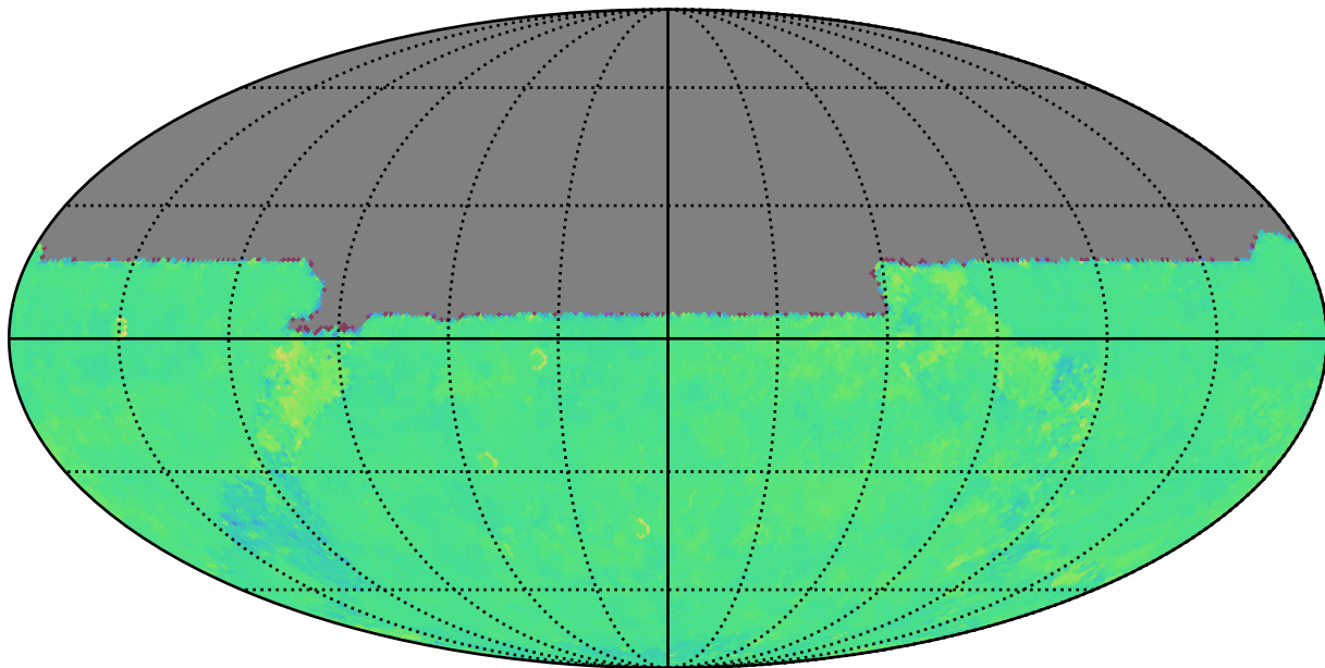
ddf_loaded_half_fl15_v3.4_10yrs u: Kuiper rotTelPos
