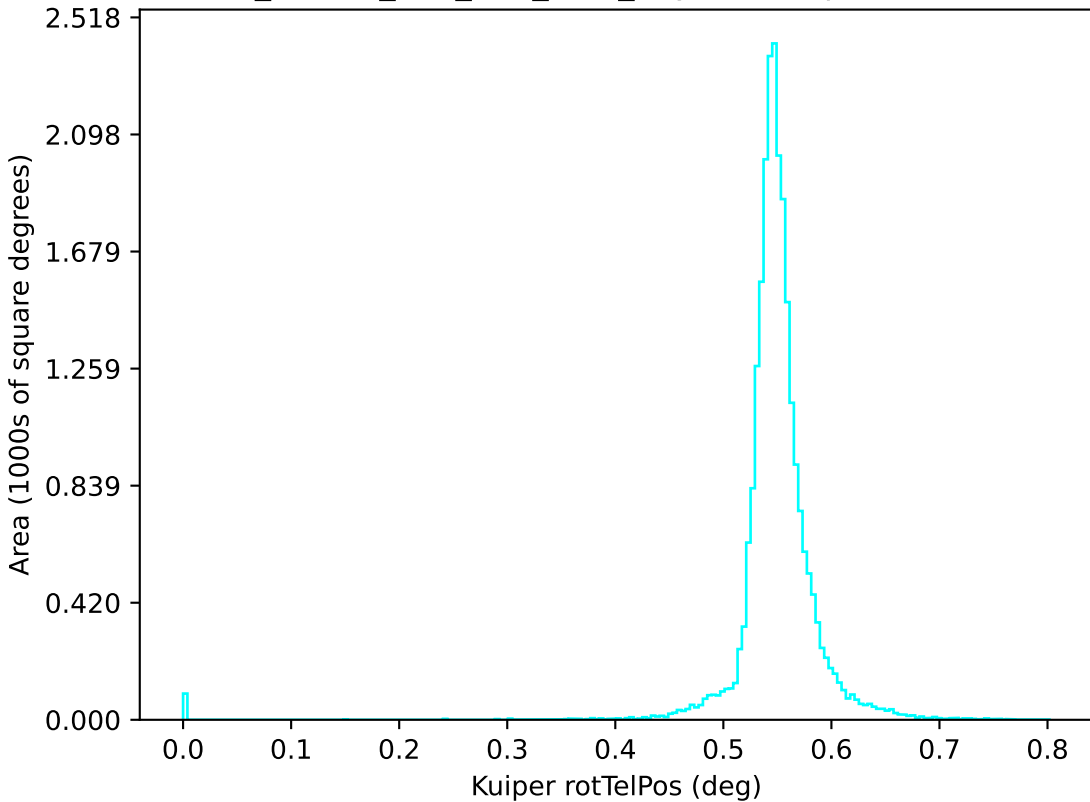
ddf_loaded_half_fl15_v3.4_10yrs u: Kuiper rotTelPos
