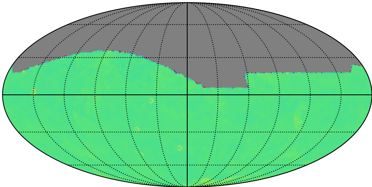
ddf_loaded_half_fl15_v3.4_10yrs r: Kuiper rotTelPos
