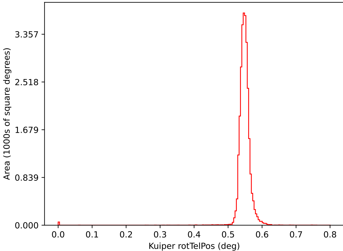
ddf_loaded_half_fl15_v3.4_10yrs i: Kuiper rotTelPos
