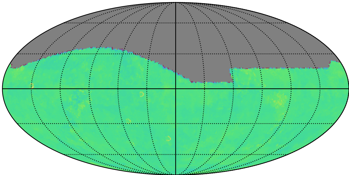
ddf_loaded_half_fl15_v3.4_10yrs g: Kuiper rotTelPos
