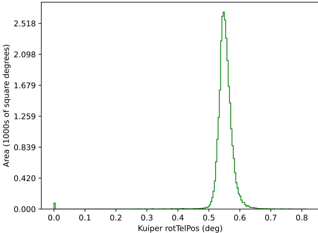
ddf_loaded_half_fl15_v3.4_10yrs g: Kuiper rotTelPos
