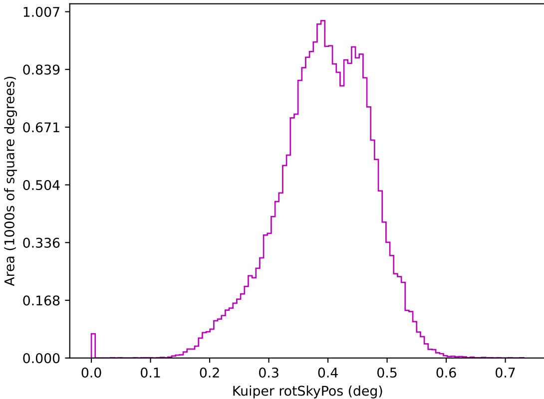
ddf_loaded_half_fl15_v3.4_10yrs z: Kuiper rotSkyPos
