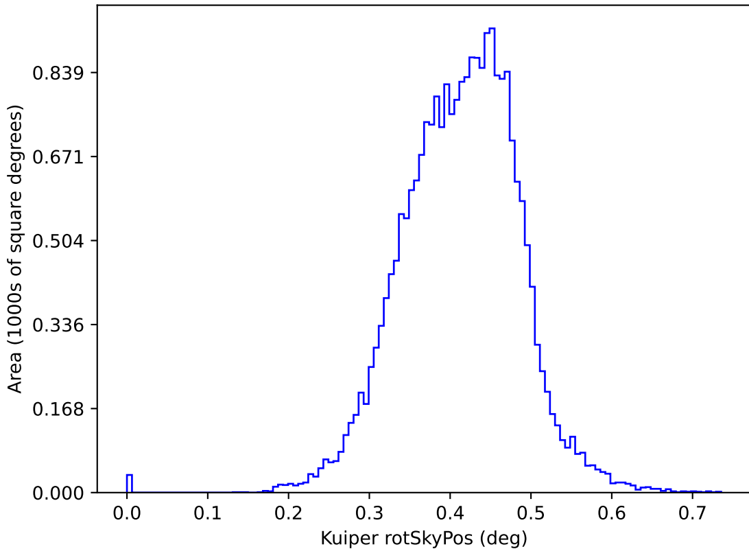
ddf_loaded_half_fl15_v3.4_10yrs y: Kuiper rotSkyPos
