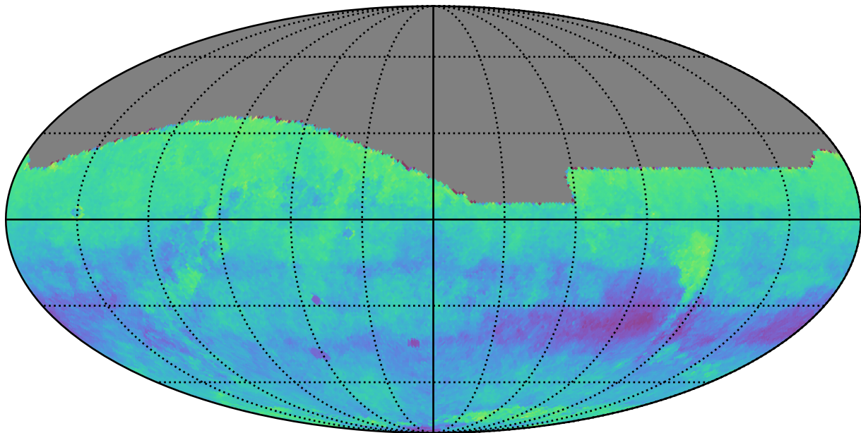
ddf_loaded_half_fl15_v3.4_10yrs r: Kuiper rotSkyPos
