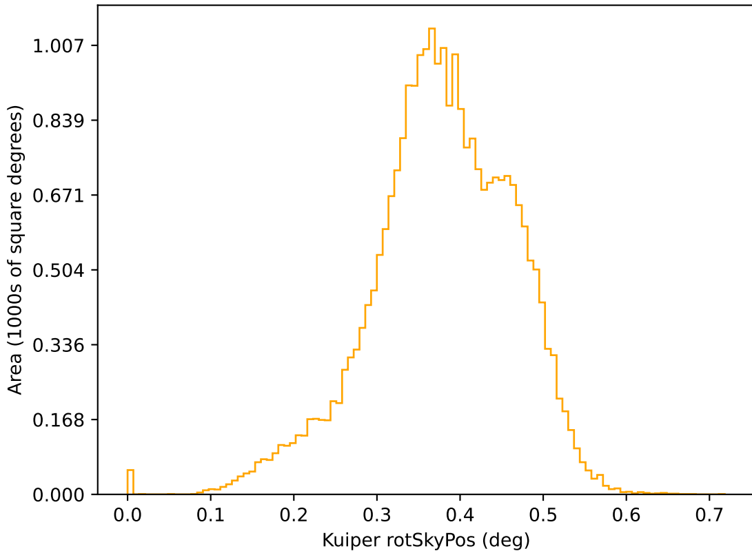
ddf_loaded_half_fl15_v3.4_10yrs r: Kuiper rotSkyPos
