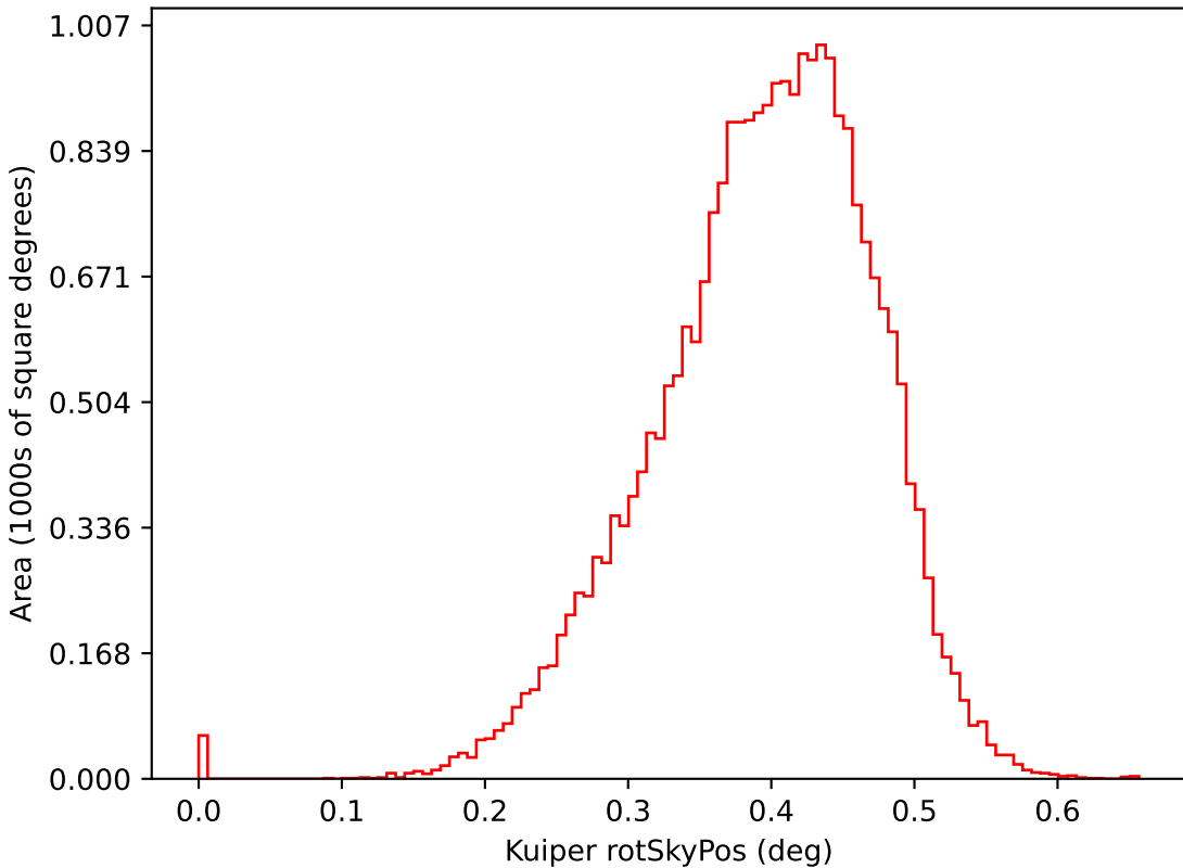
ddf_loaded_half_fl15_v3.4_10yrs i: Kuiper rotSkyPos
