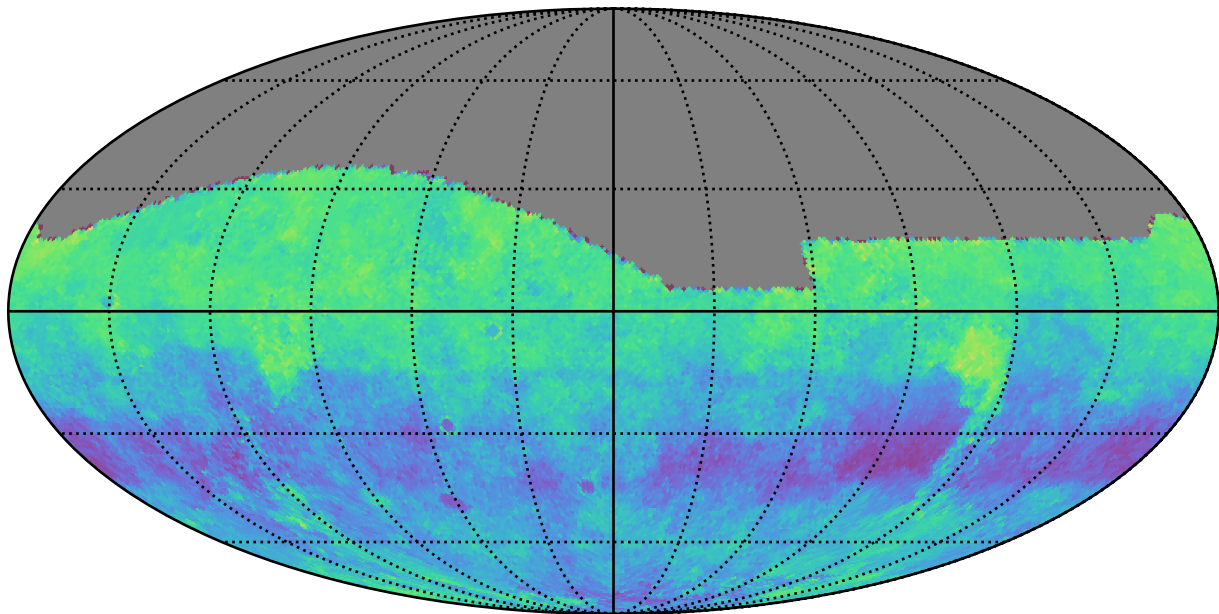
ddf_loaded_half_fl15_v3.4_10yrs g: Kuiper rotSkyPos
