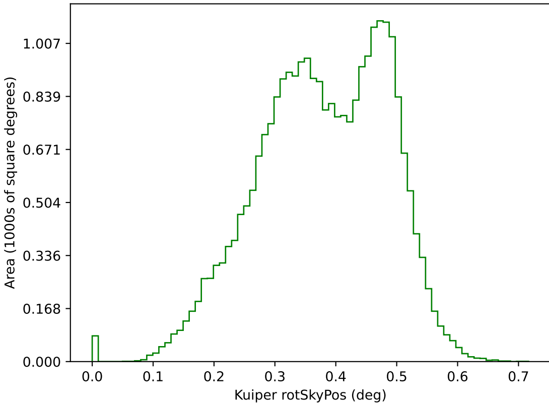
ddf_loaded_half_fl15_v3.4_10yrs g: Kuiper rotSkyPos
