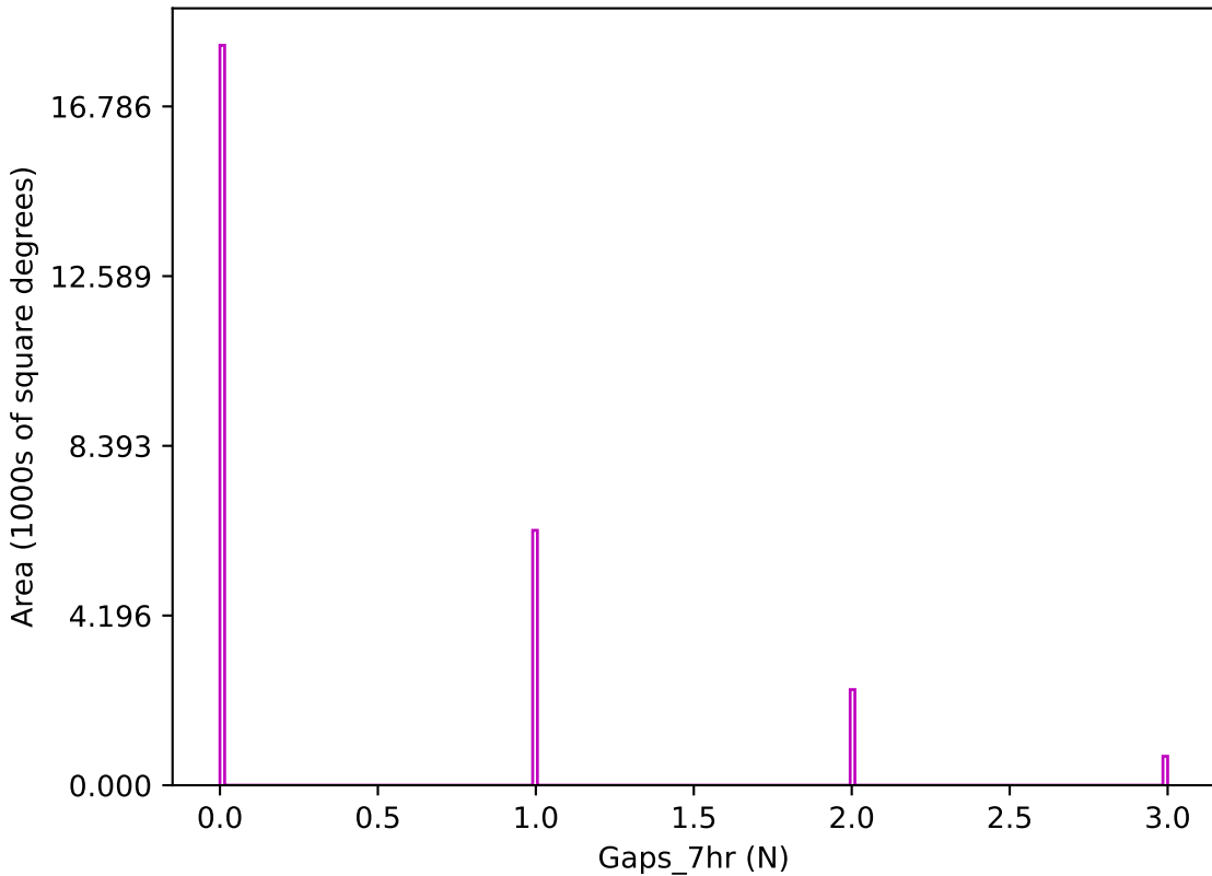
ddf_loaded_half_fl15_v3.4_10yrs z band: Gaps_7hr
