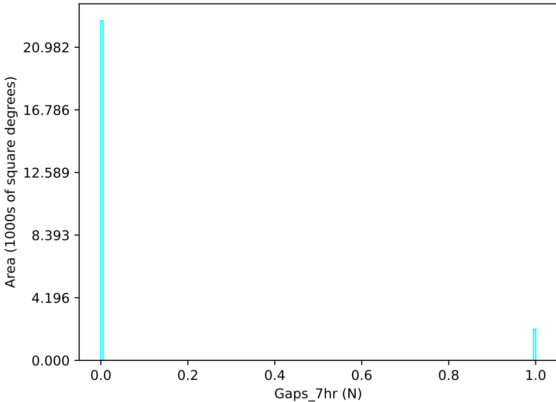
ddf_loaded_half_fl15_v3.4_10yrs u band: Gaps_7hr
