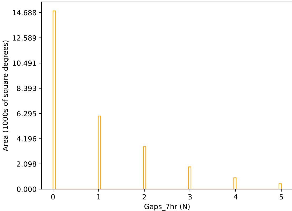
ddf_loaded_half_fl15_v3.4_10yrs r band: Gaps_7hr
