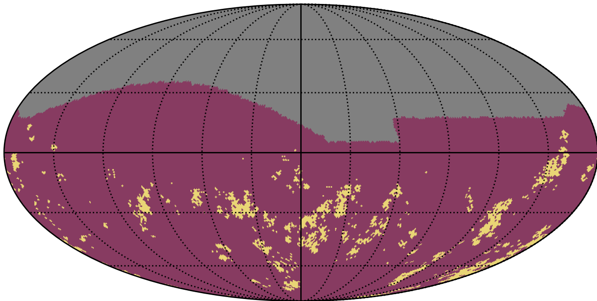
ddf_loaded_half_fl15_v3.4_10yrs g band: Gaps_7hr
