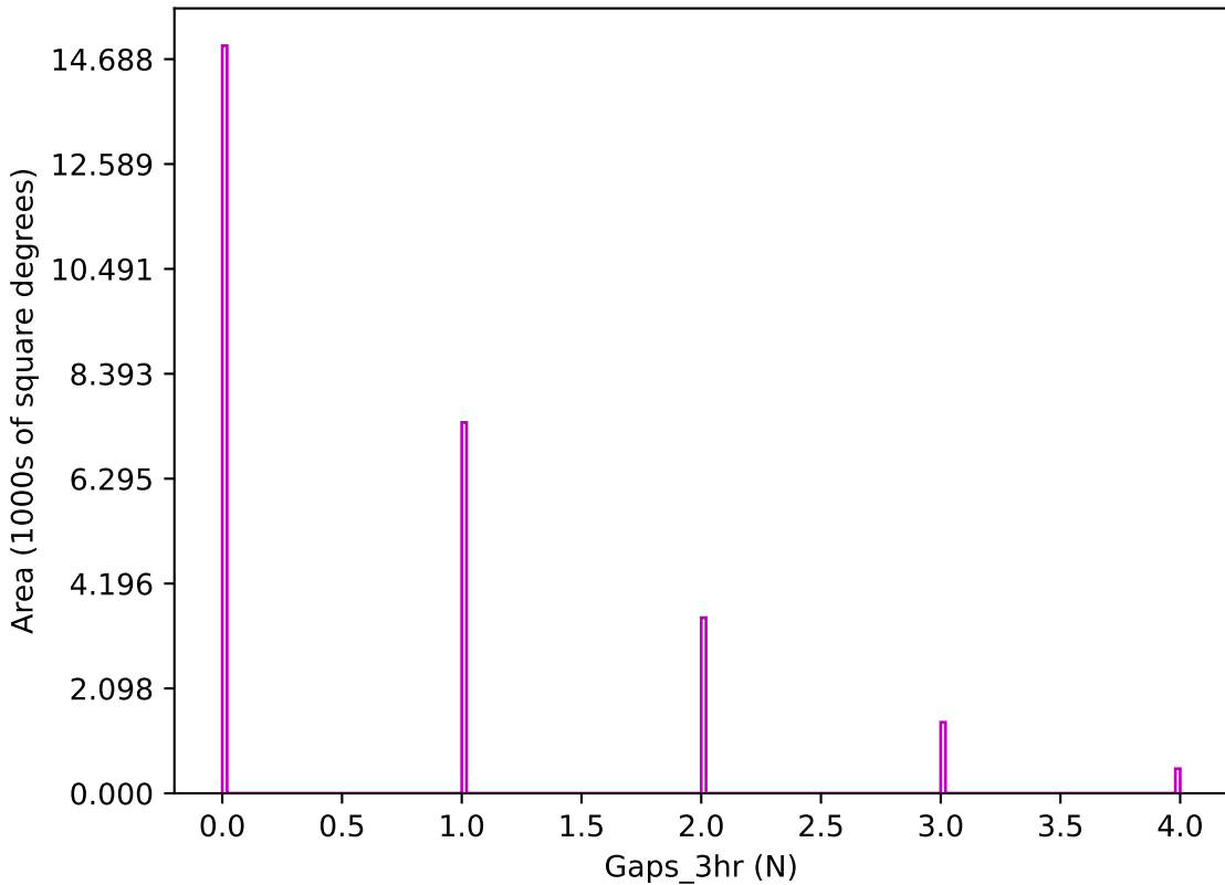
ddf_loaded_half_fl15_v3.4_10yrs z band: Gaps_3hr
