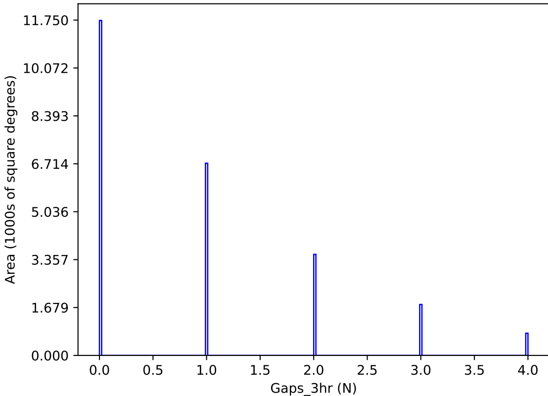
ddf_loaded_half_fl15_v3.4_10yrs y band: Gaps_3hr
