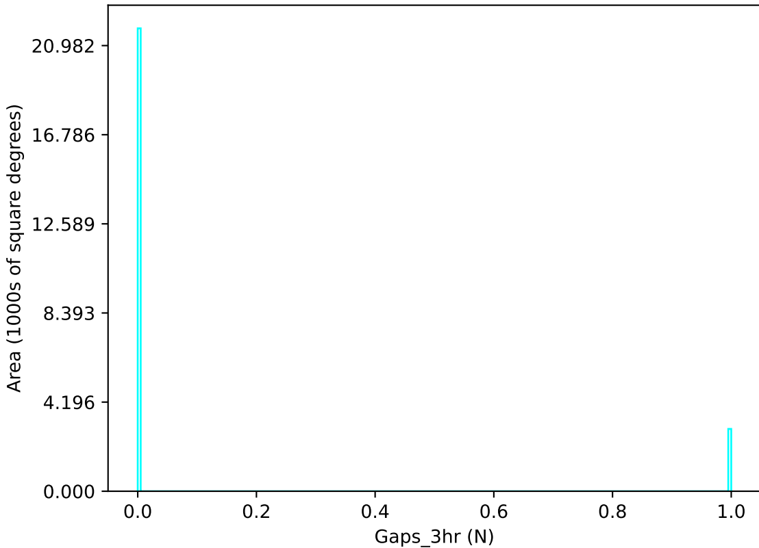
ddf_loaded_half_fl15_v3.4_10yrs u band: Gaps_3hr
