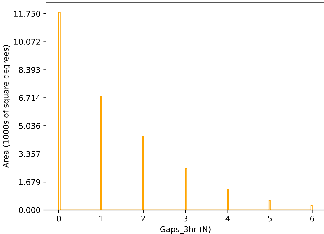
ddf_loaded_half_fl15_v3.4_10yrs r band: Gaps_3hr
