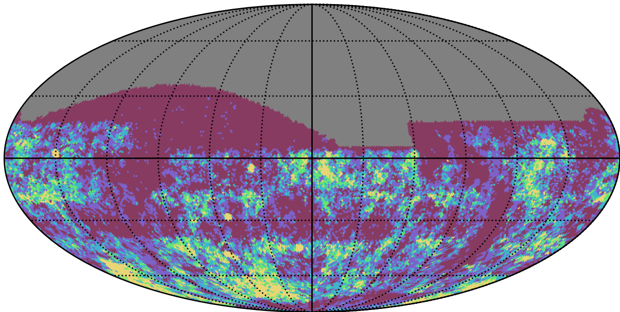
ddf_loaded_half_fl15_v3.4_10yrs i band: Gaps_3hr
