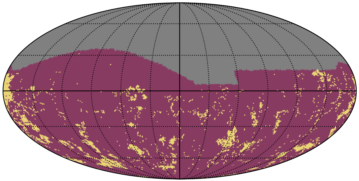
ddf_loaded_half_fl15_v3.4_10yrs g band: Gaps_3hr
