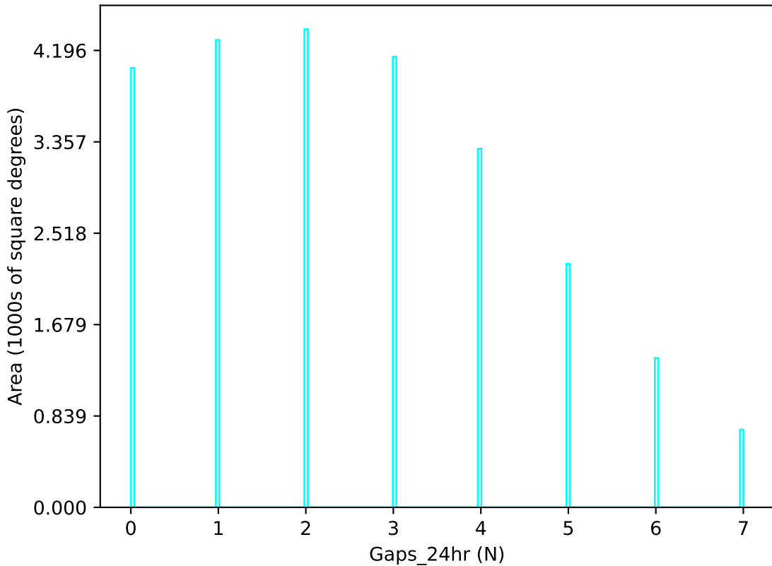
ddf_loaded_half_fl15_v3.4_10yrs u band: Gaps_24hr
