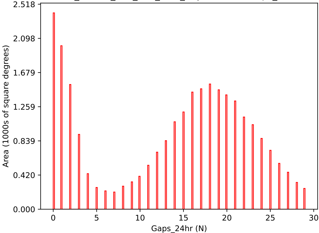
ddf_loaded_half_fl15_v3.4_10yrs i band: Gaps_24hr
