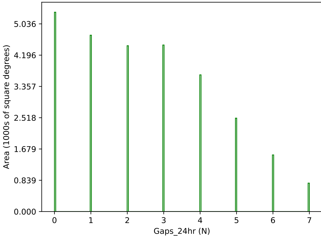
ddf_loaded_half_fl15_v3.4_10yrs g band: Gaps_24hr
