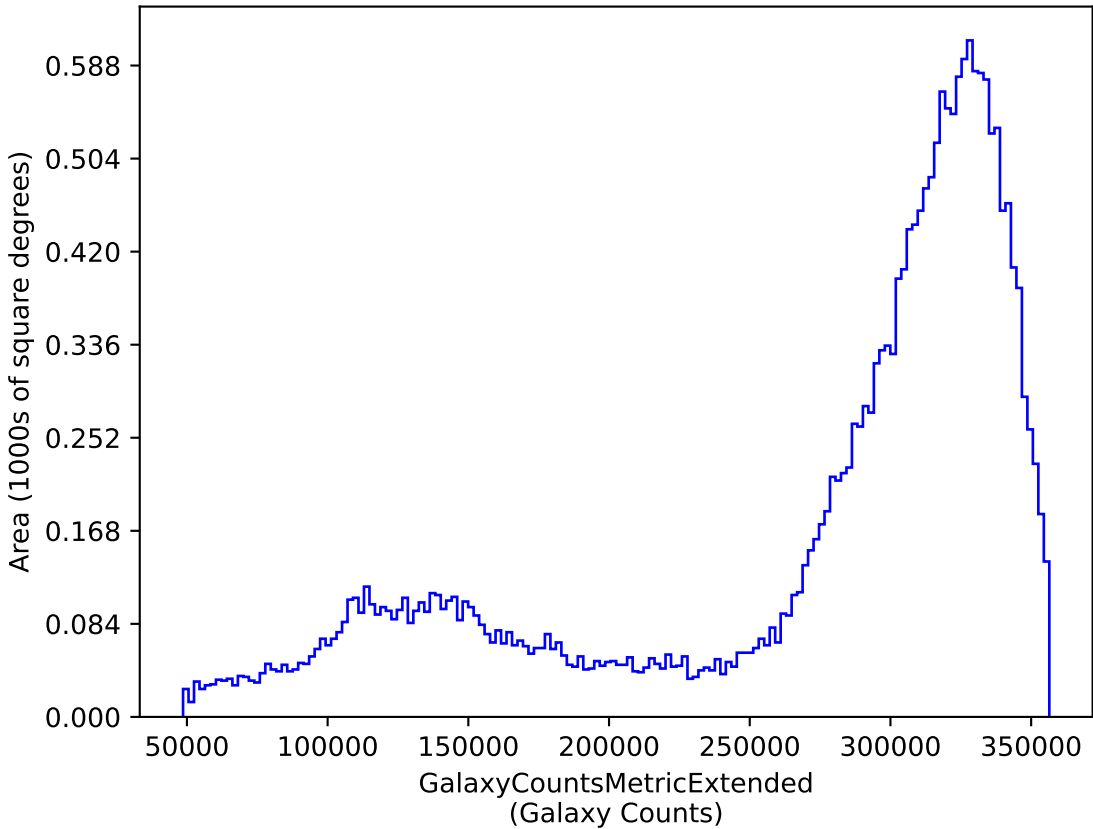
ddf_loaded_half_fl15_v3.4_10yrs y: GalaxyCountsMetricExtended
