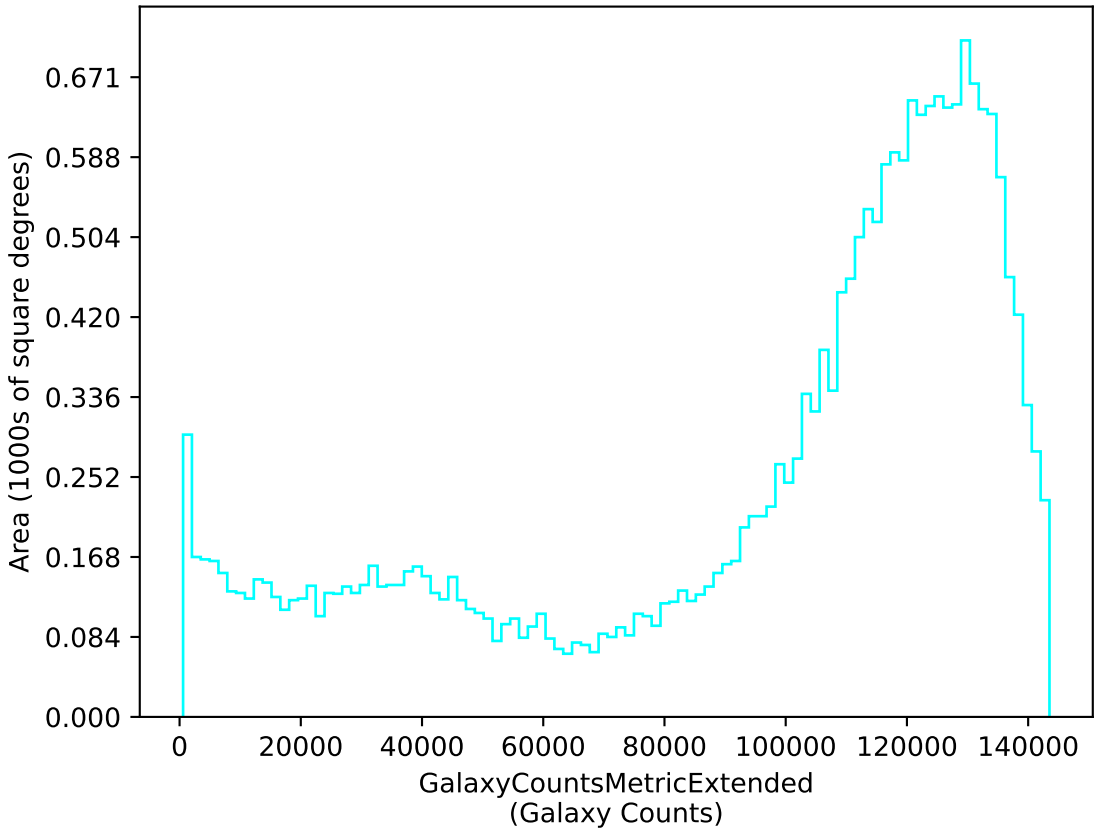
ddf_loaded_half_fl15_v3.4_10yrs u: GalaxyCountsMetricExtended
