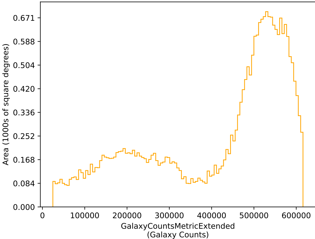
ddf_loaded_half_fl15_v3.4_10yrs r: GalaxyCountsMetricExtended
