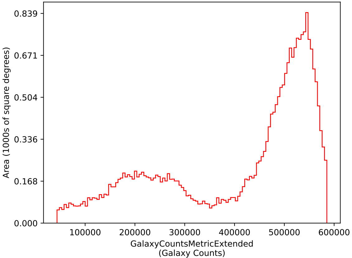
ddf_loaded_half_fl15_v3.4_10yrs i: GalaxyCountsMetricExtended
