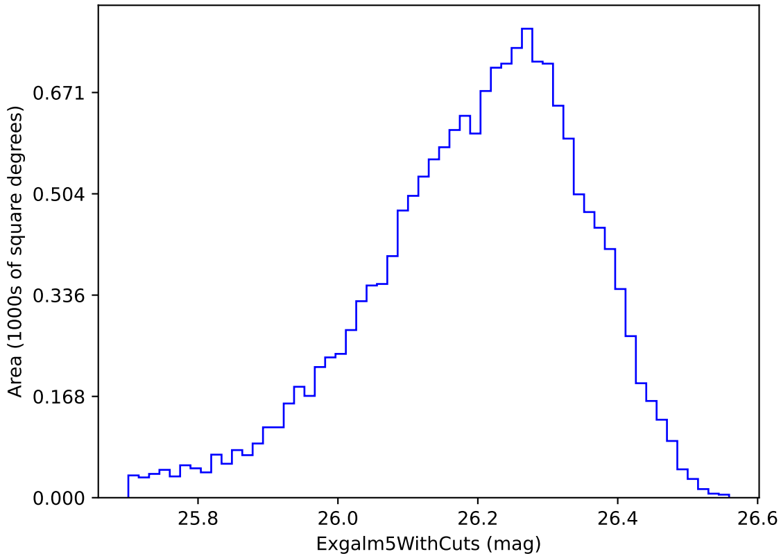
ddf_loaded_half_fl15_v3.4_10yrs i band non-DD year 7: Exgalml5WithCuts
