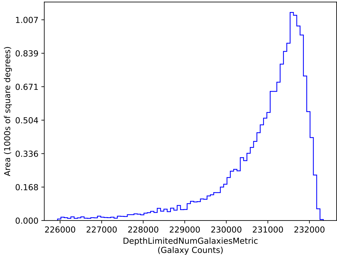
ddf_loaded_half_fl15_v3.4_10yrs i band galaxies non-DD: DepthLimitedNumGalaxiesMetric
